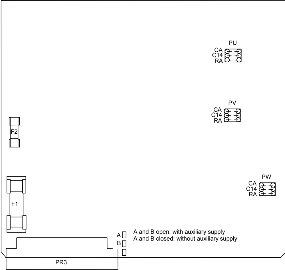
Power board adjustment for amplifier types 220/70 and 220/100
