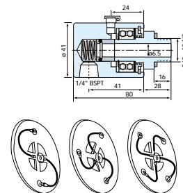
1/4" ROTO Coupling part No 40067-730
