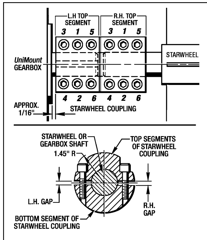
Figure 3.2 - Installing Drive Coupling
