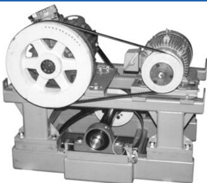
Specifically designed ultra quick Posidyne Clutch/Brake with flywheel and welded tubular base completely assembled.
