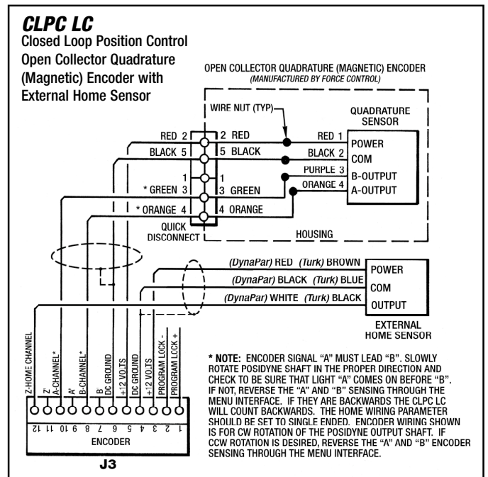
Figure 2 - Wiring Diagram - Terminal Block #J3 (With External Home Sensor)
