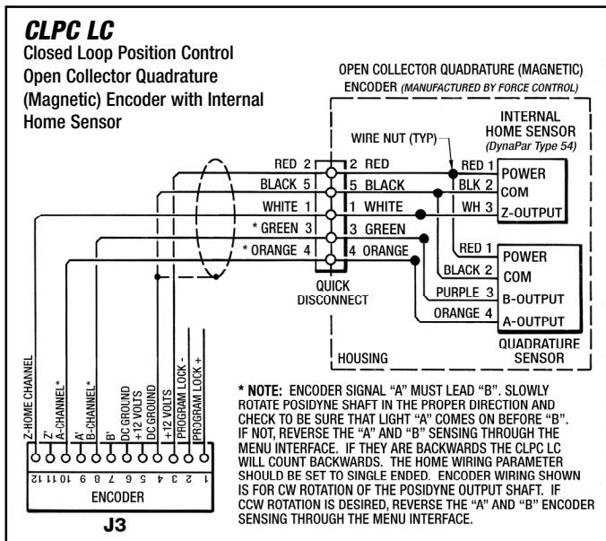
Figure 1 - Wiring Diagram - Terminal Block #J3 (With Internal Home Sensor)
