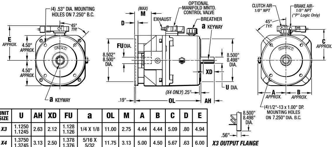
Figure 2 - Dimensions
