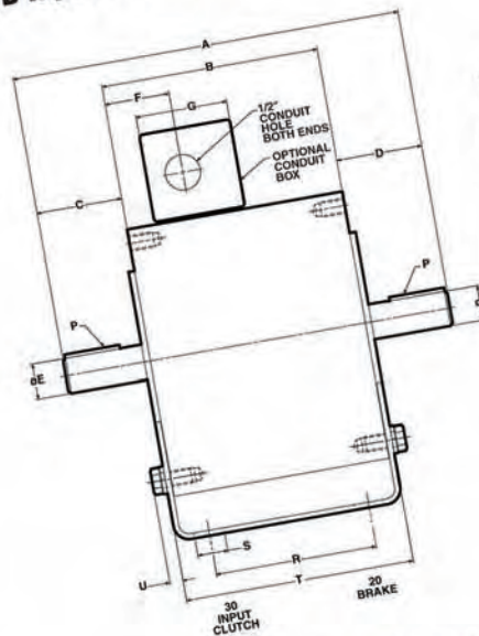
Dimensions (Blue shaded areas indicate GEN 2 design)
