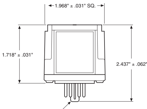
STD. OCTAL KEYED PLUG
