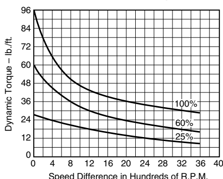
Size 650 Maximum Speed 3,600 rpm Static Torque 95 lb./ft.
