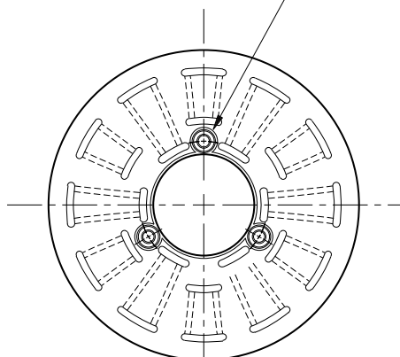
ARMATURE VIEW
