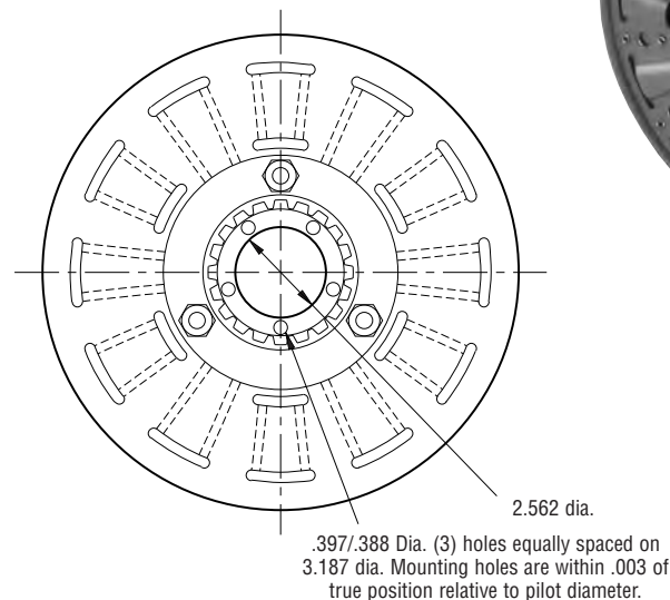
ARMATURE VIEW
