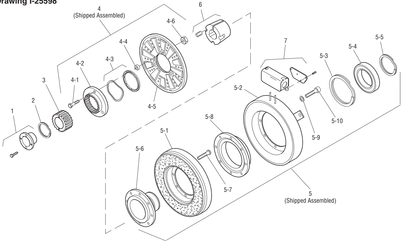
Drawing I-25598
