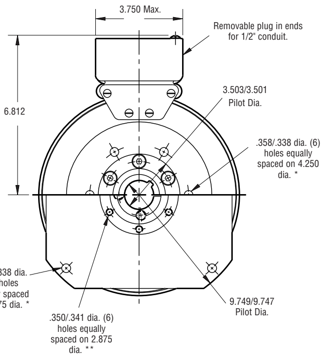
FIELD VIEW
