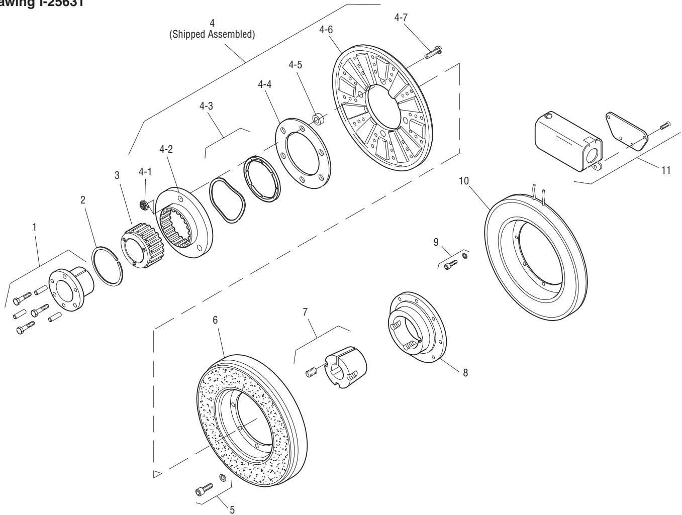
Drawing I-25631
