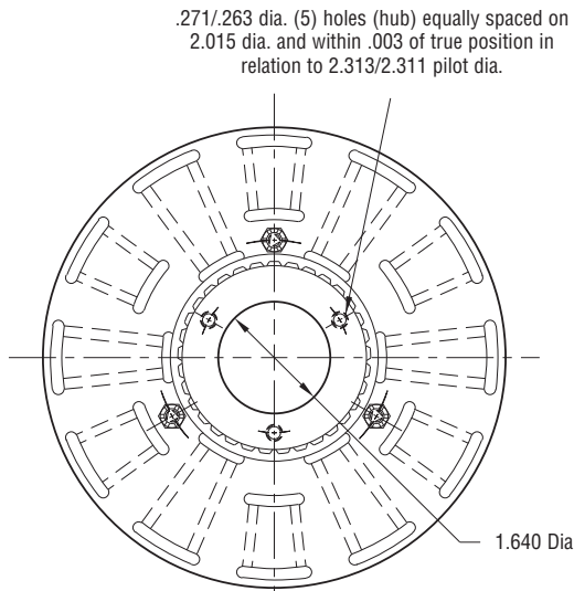
ARMATURE VIEW
