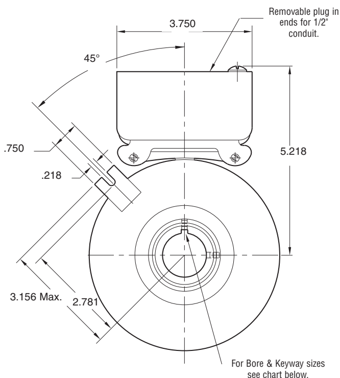
FIELD VIEW
