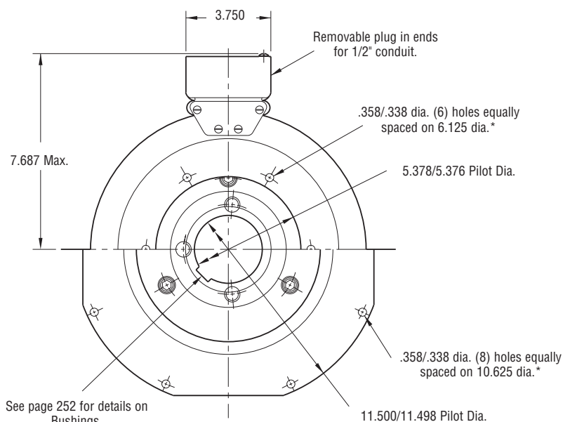
MAGNET VIEW
