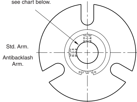
ARMATURE VIEW
