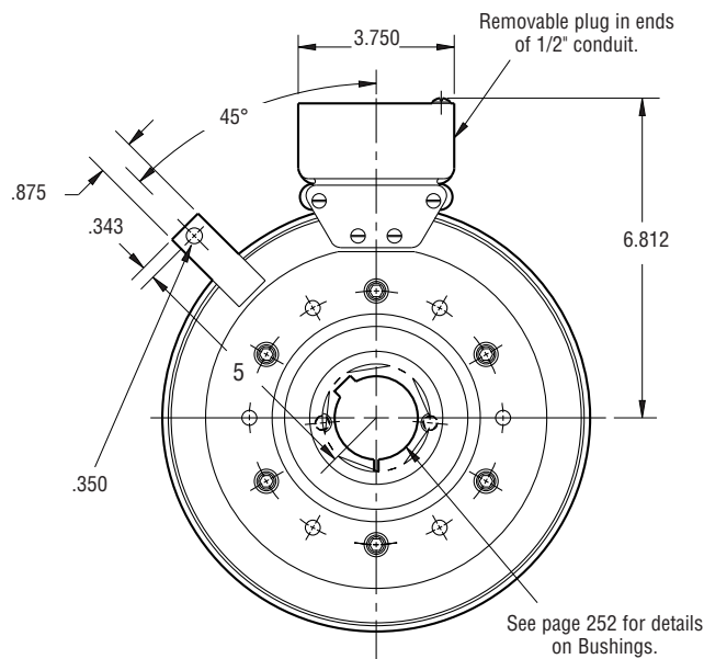
FIELD VIEW
