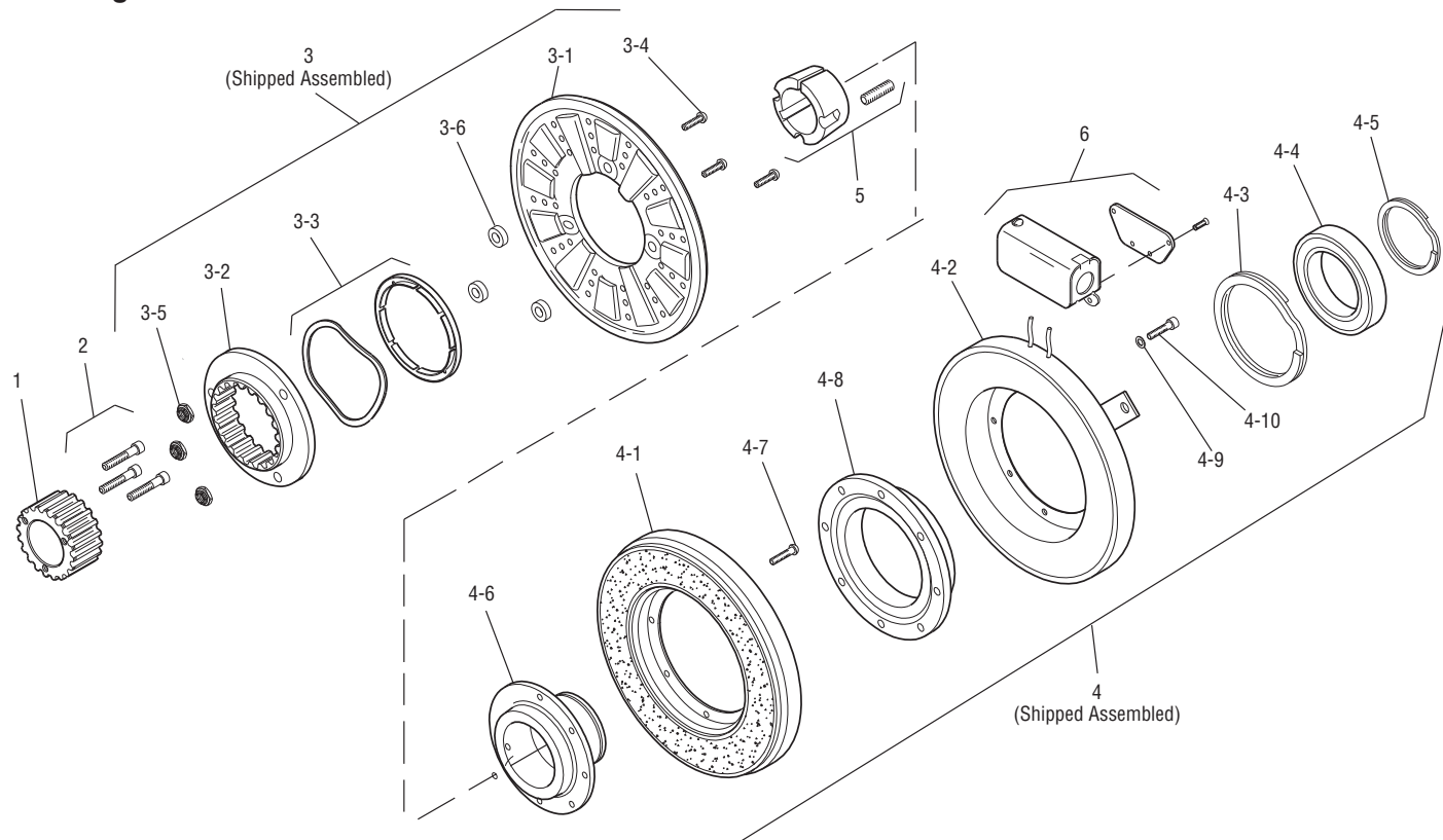
Drawing I-25622
