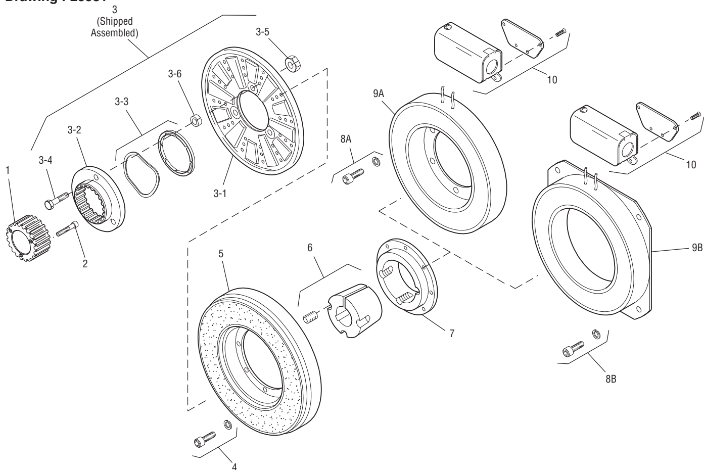
Drawing I-25581
