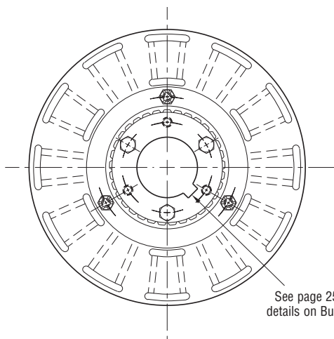
ARMATURE VIEW
