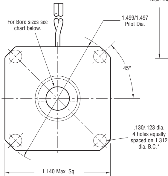
FIELD VIEW
