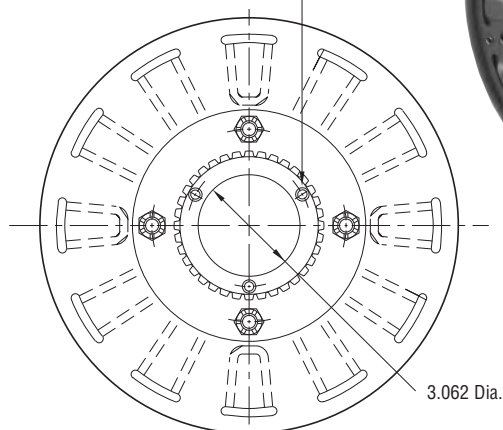
ARMATURE VIEW
