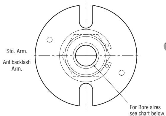
ARMATURE VIEW
