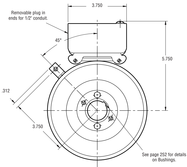
FIELD VIEW
