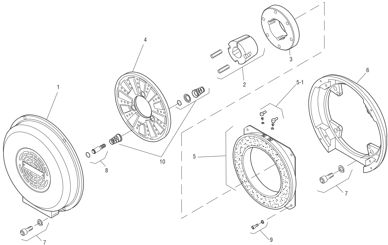
Drawing I-25572
