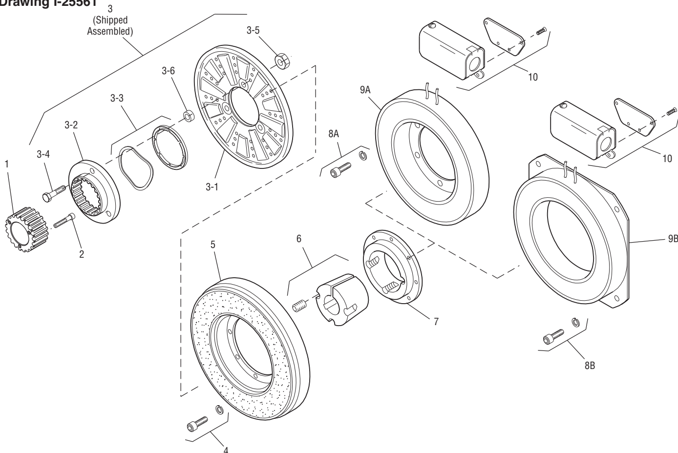
Drawing I-25561
