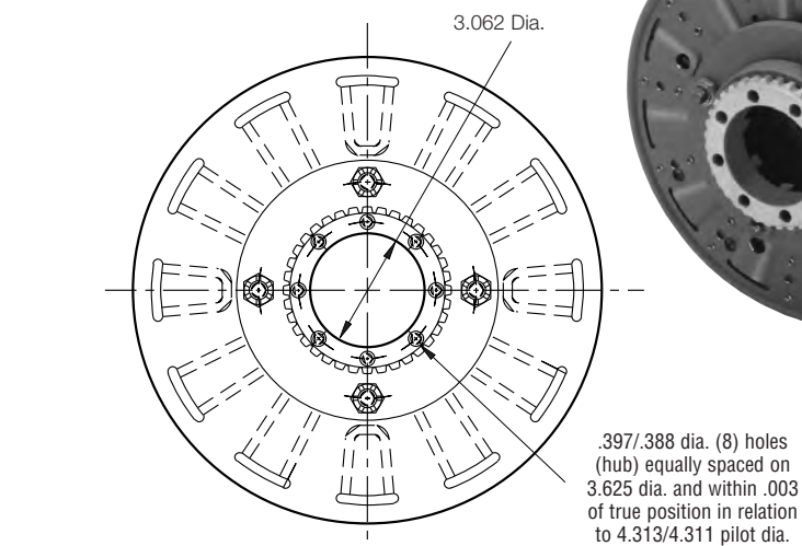
ARMATURE VIEW
