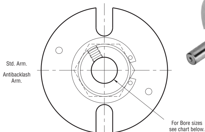
ARMATURE VIEW
