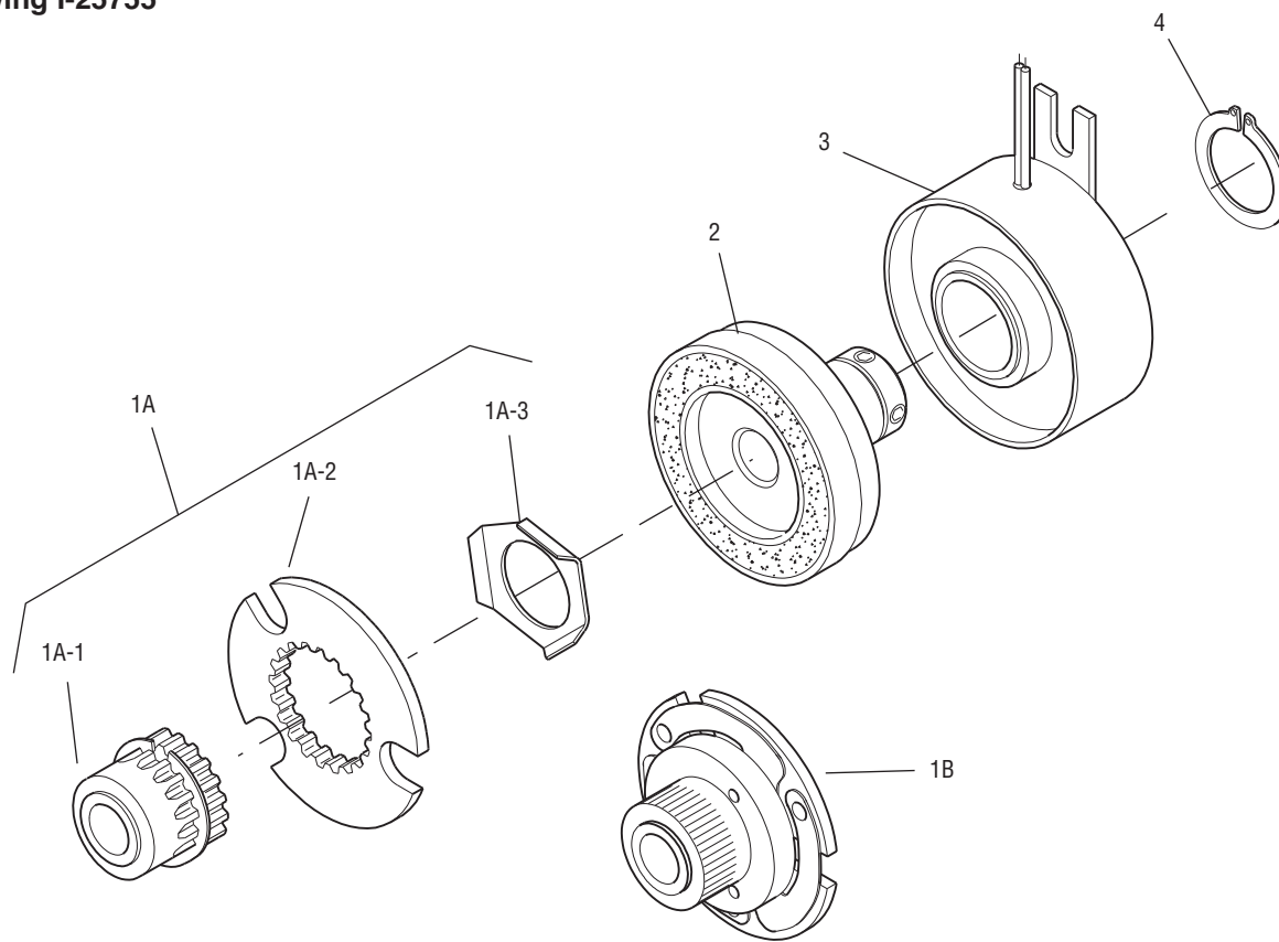
Drawing I-25755
