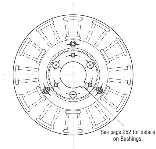
ARMATURE VIEW
