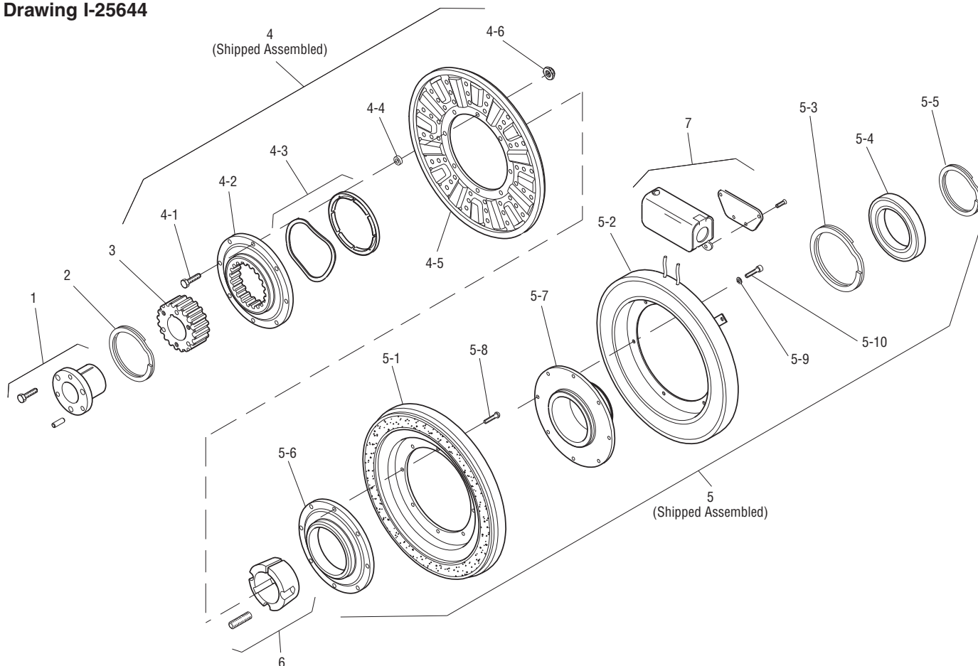
Drawing I-25644
