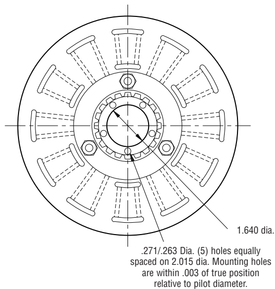
ARMATURE VIEW
