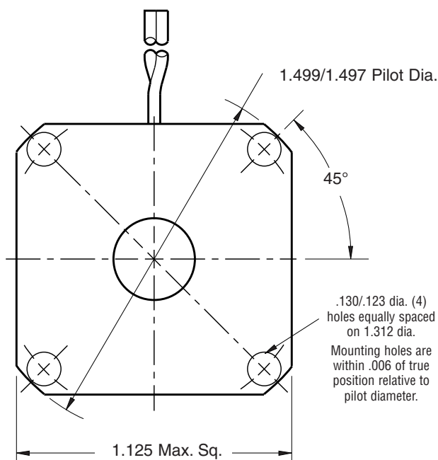
MAGNET VIEW
