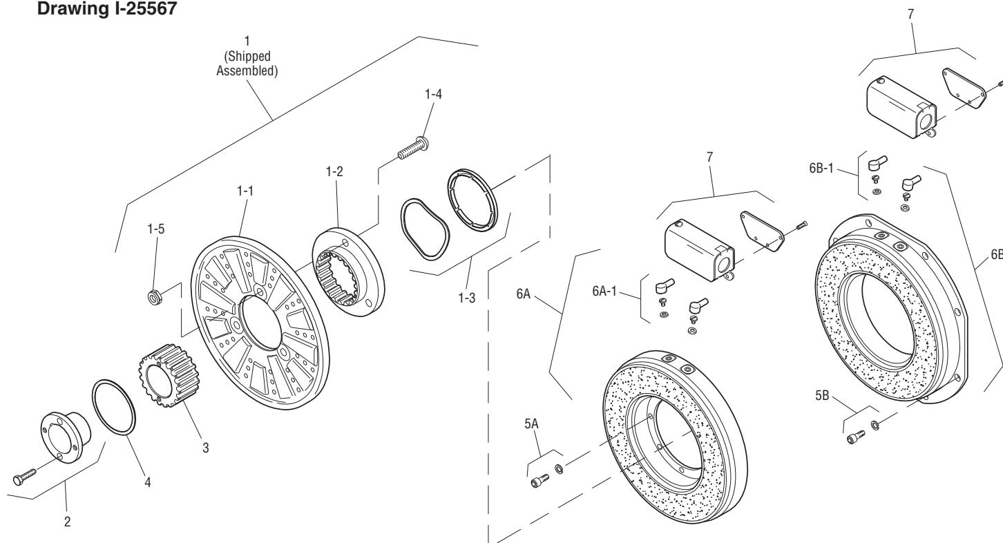
Drawing I-25567
