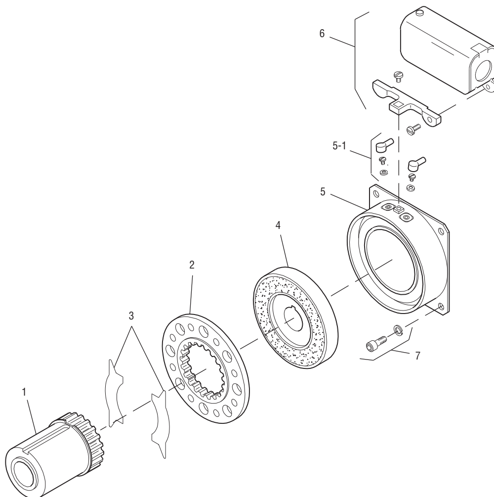
Drawing I-25695
