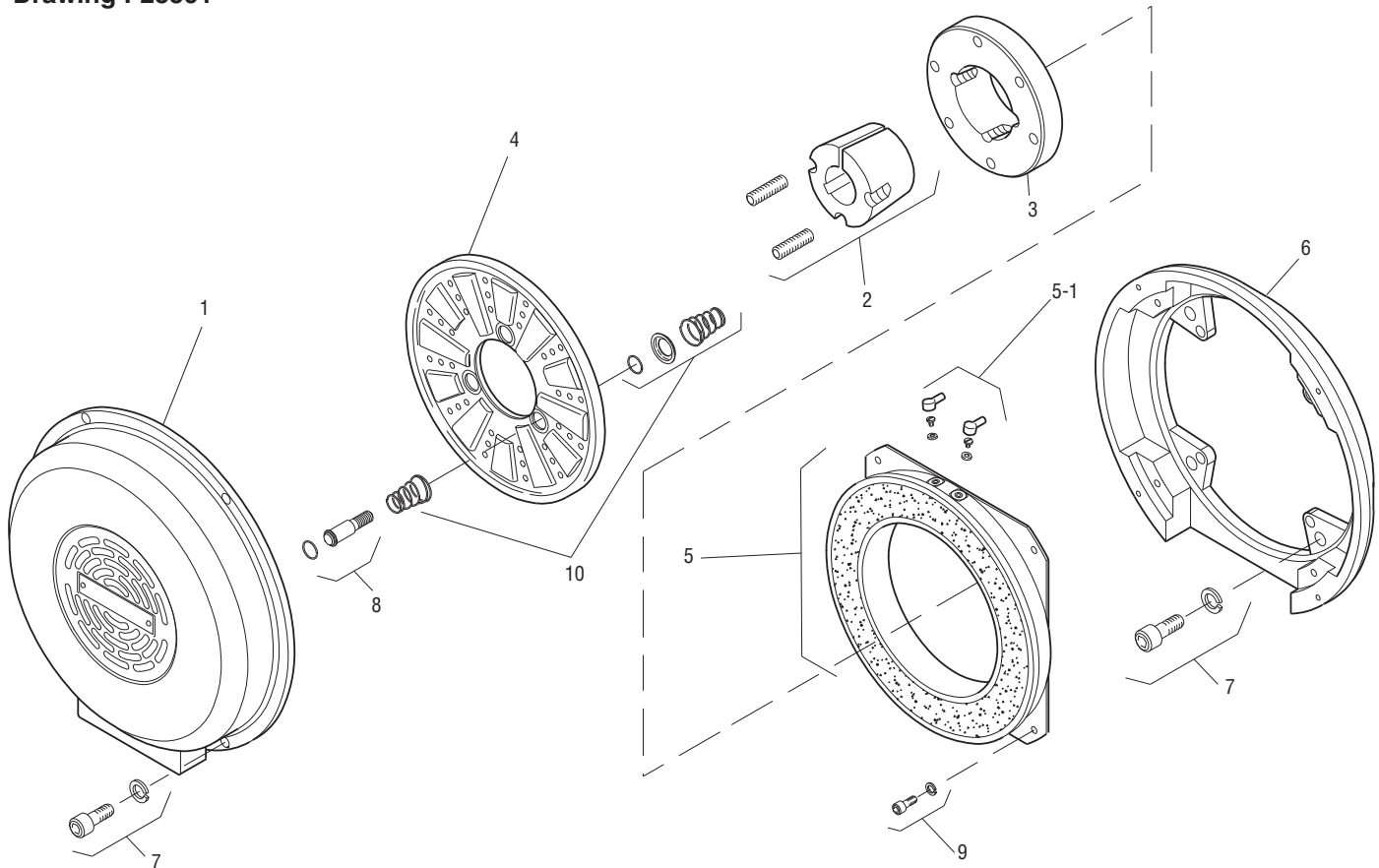
Drawing I-25591
