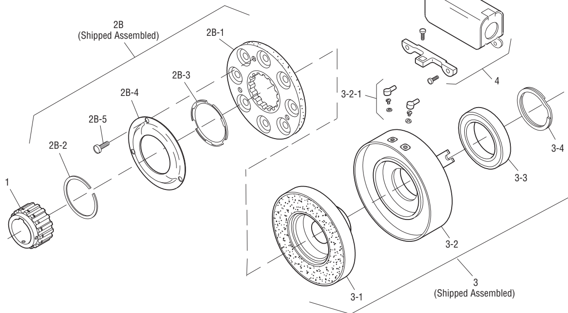
Drawing I-25541
