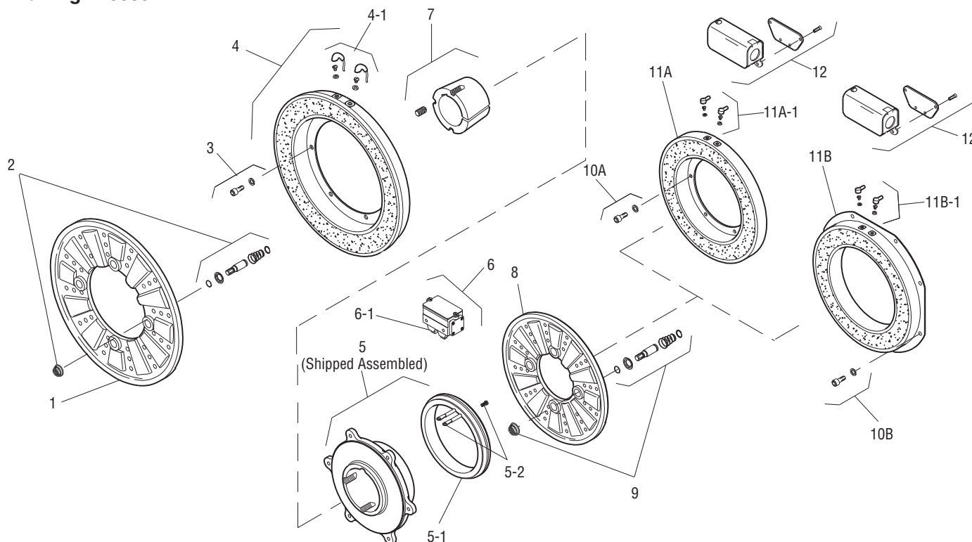
Drawing I-25635
