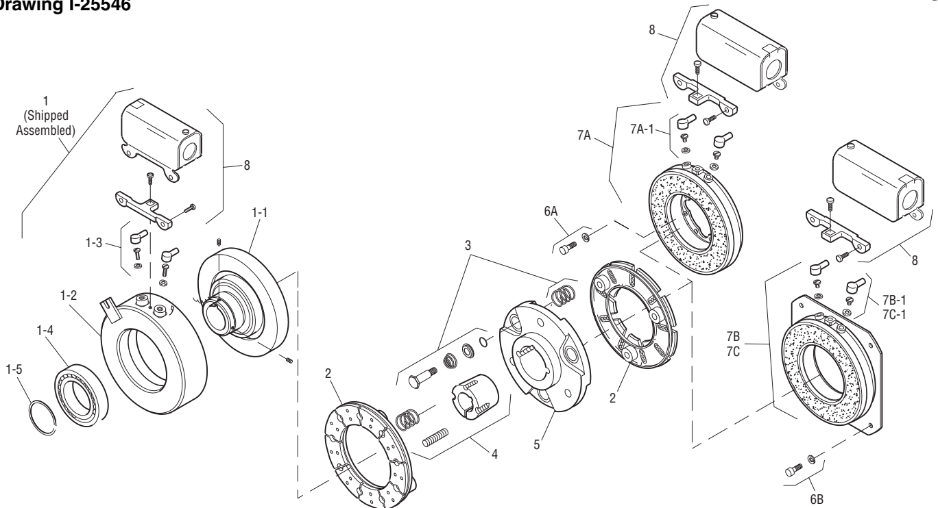
Drawing I-25546
