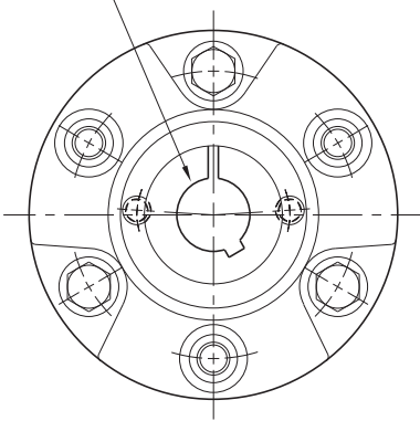
HUB VIEW
