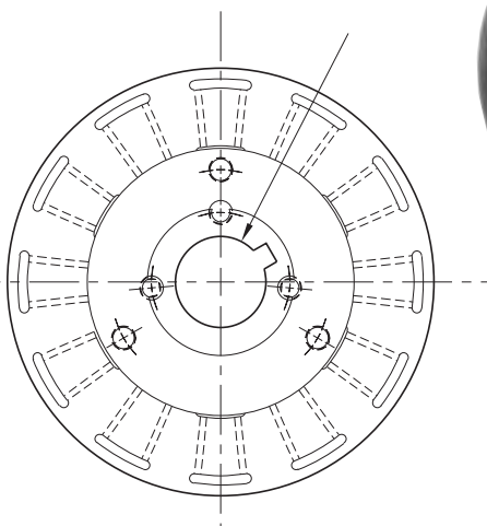
ARMATURE VIEW
