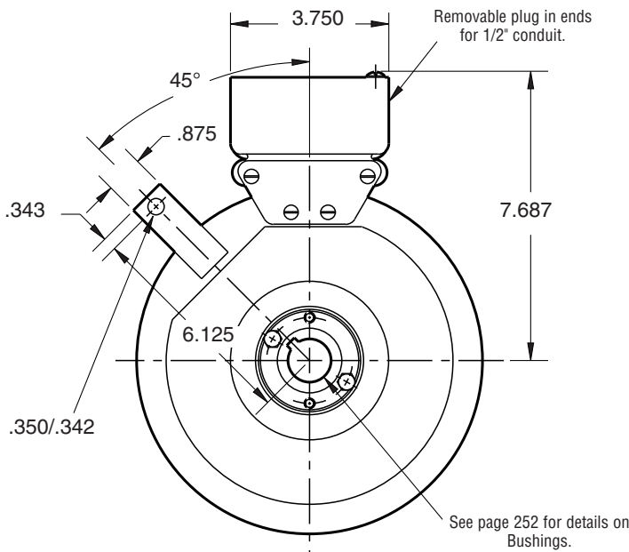
FIELD VIEW
