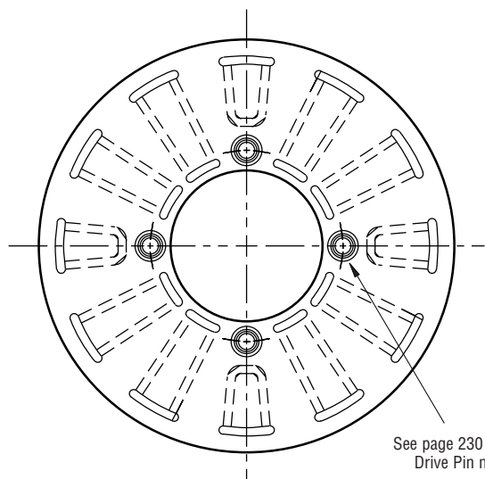
ARMATURE VIEW
