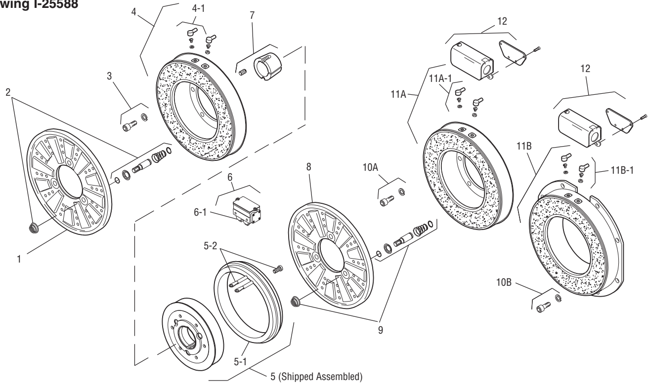
Drawing I-25588
