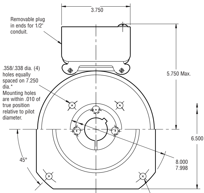
ARMATURE VIEW
