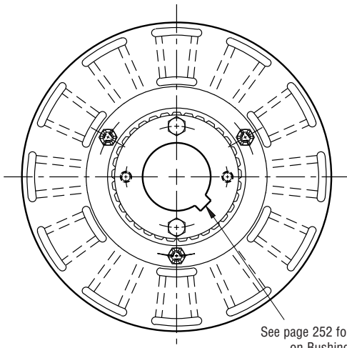
ARMATURE VIEW
