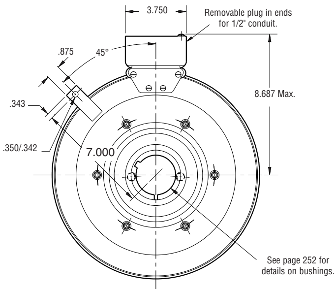
FIELD VIEW
