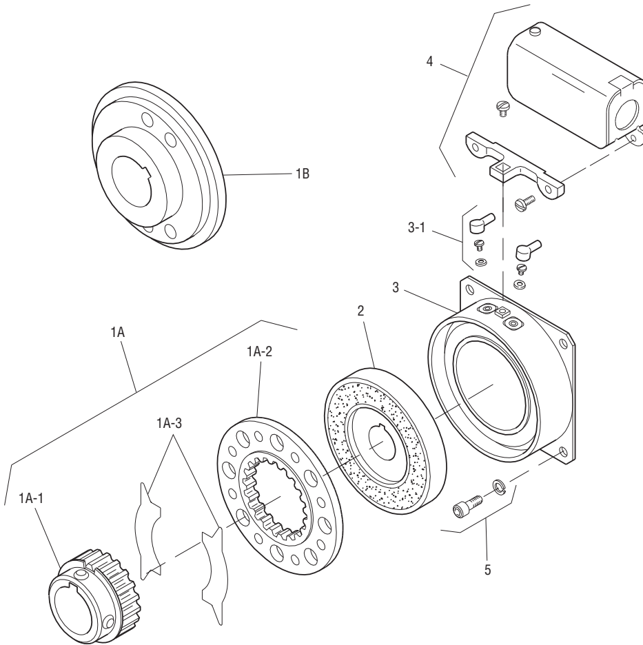
Drawing I-25697
