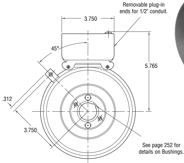
FIELD VIEW
