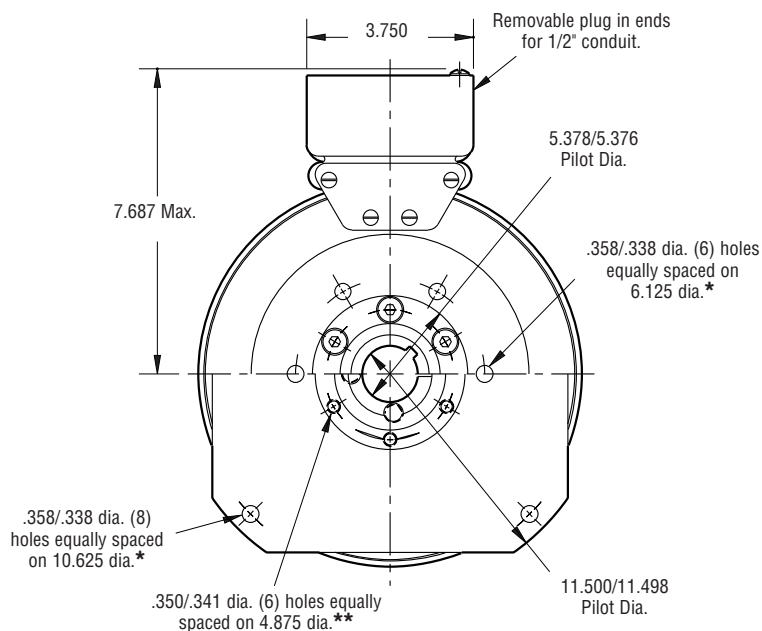
FIELD VIEW
