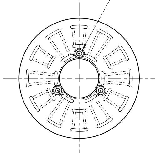
ARMATURE VIEW
