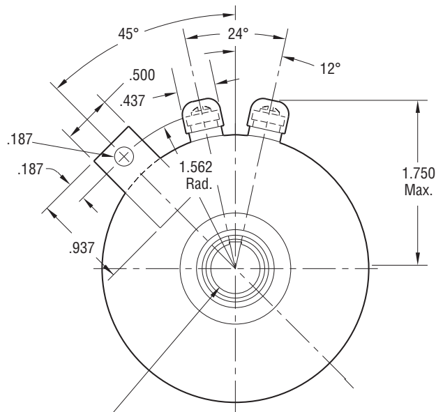
ARMATURE VIEW
