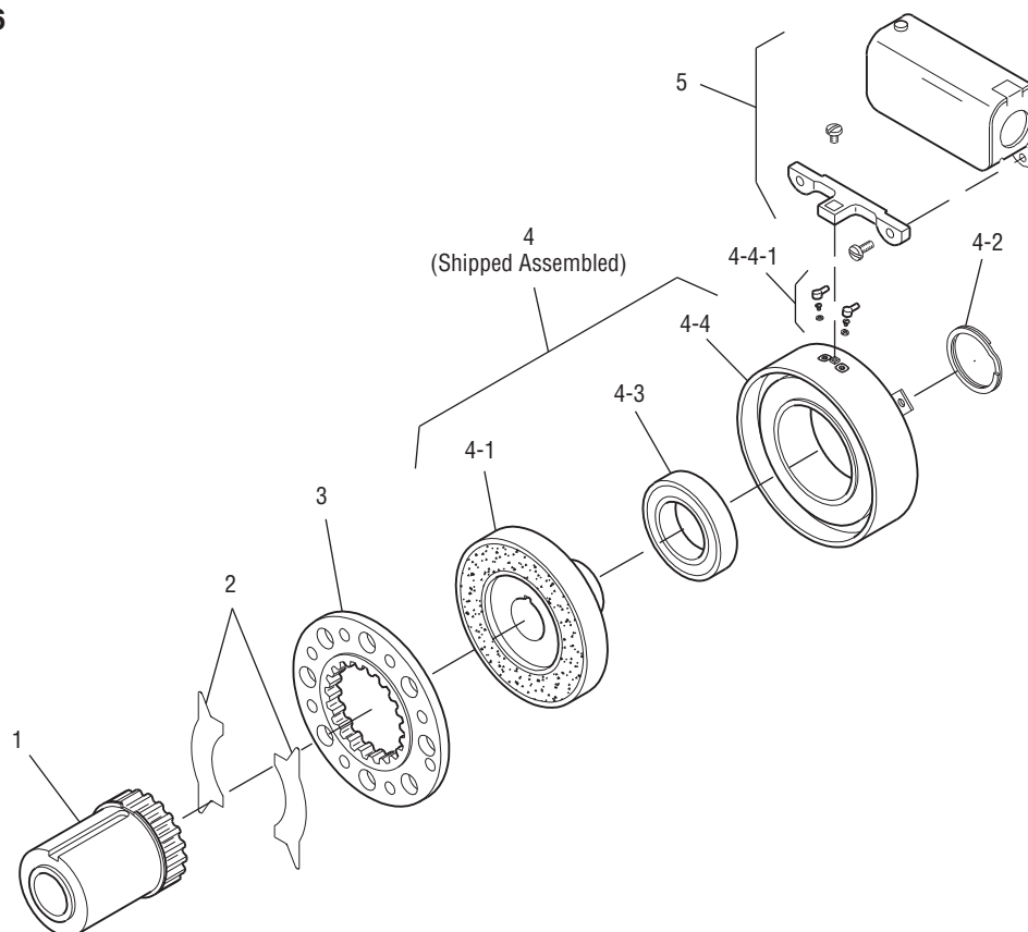
Drawing I-25696
