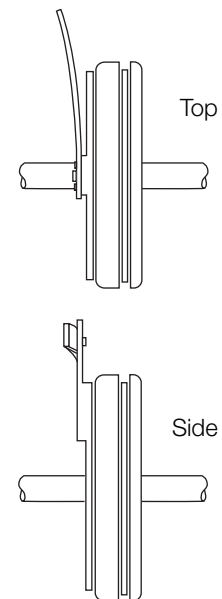
Figure 2 Rigid Member with Slot Straddling Tab (Preferred)
