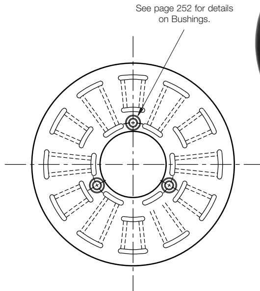
ARMATURE VIEW
