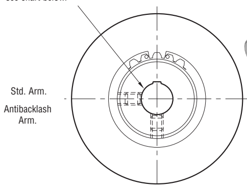
ARMATURE VIEW
