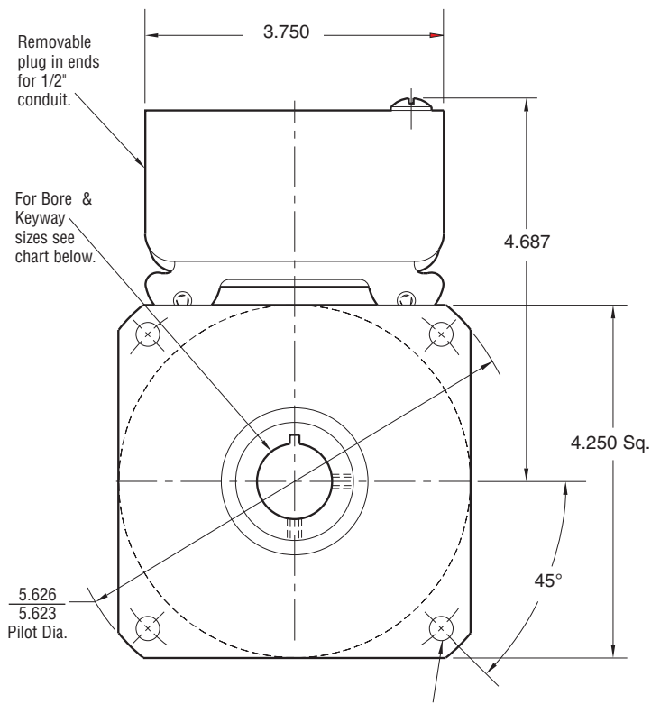
ARMATURE VIEW
