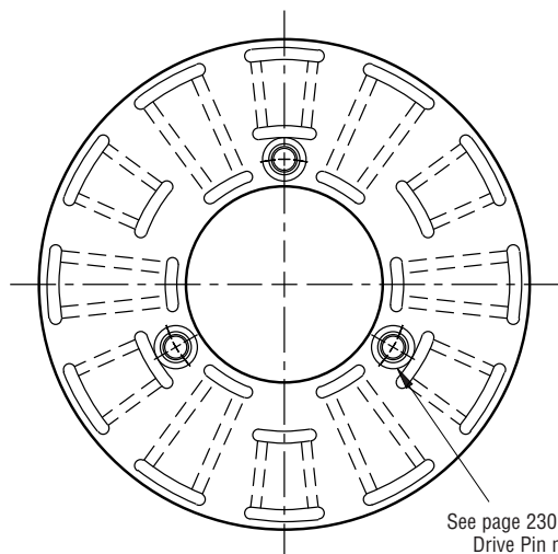
ARMATURE VIEW
