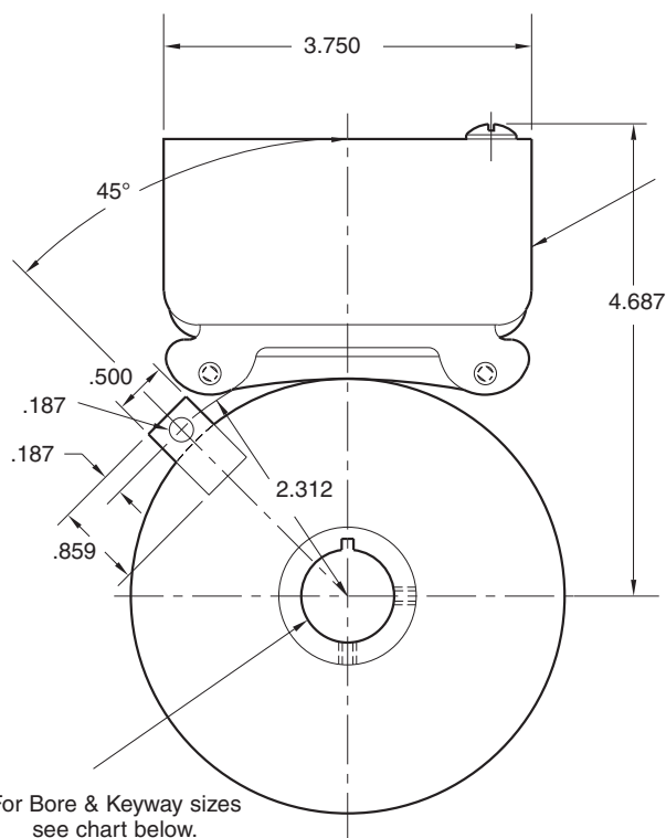
FIELD VIEW
