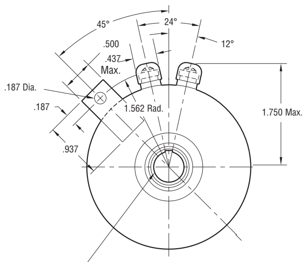
FIELD VIEW
