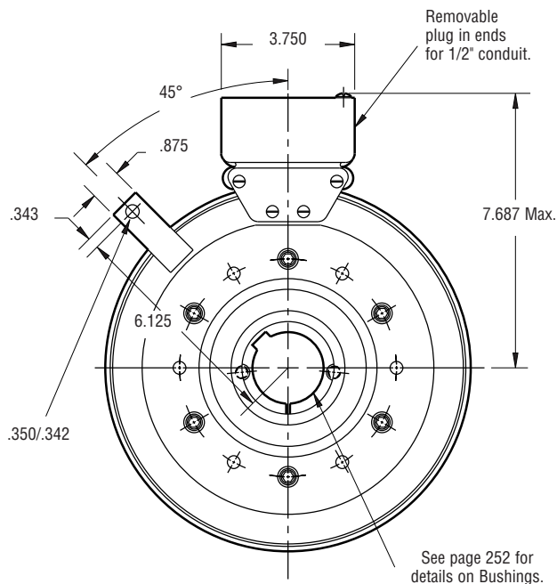
FIELD VIEW
