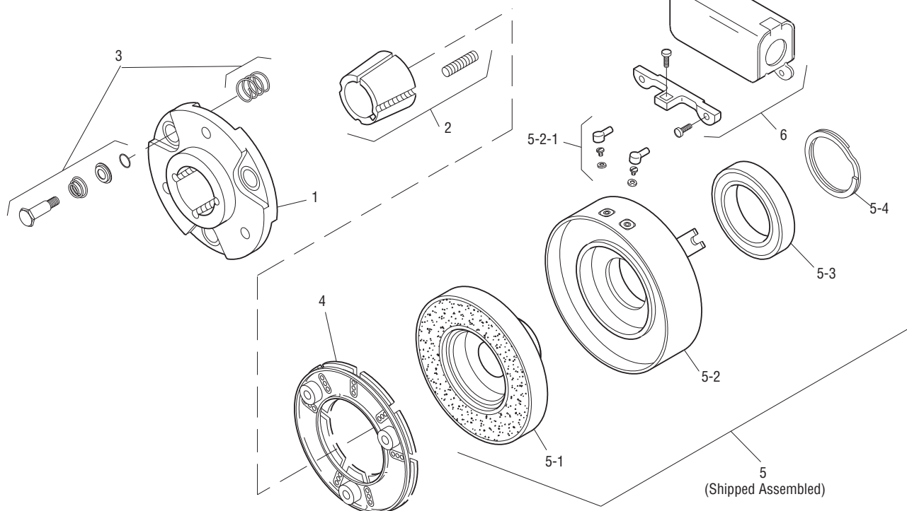
Drawing I-25540
