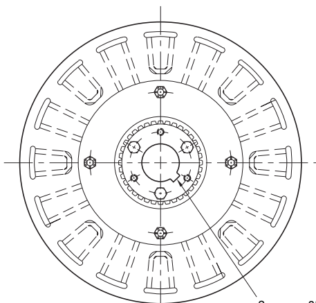
ARMATURE VIEW
