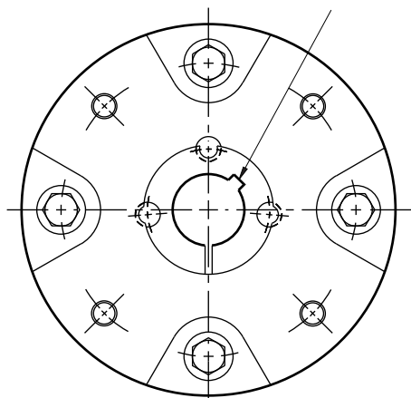
HUB VIEW
