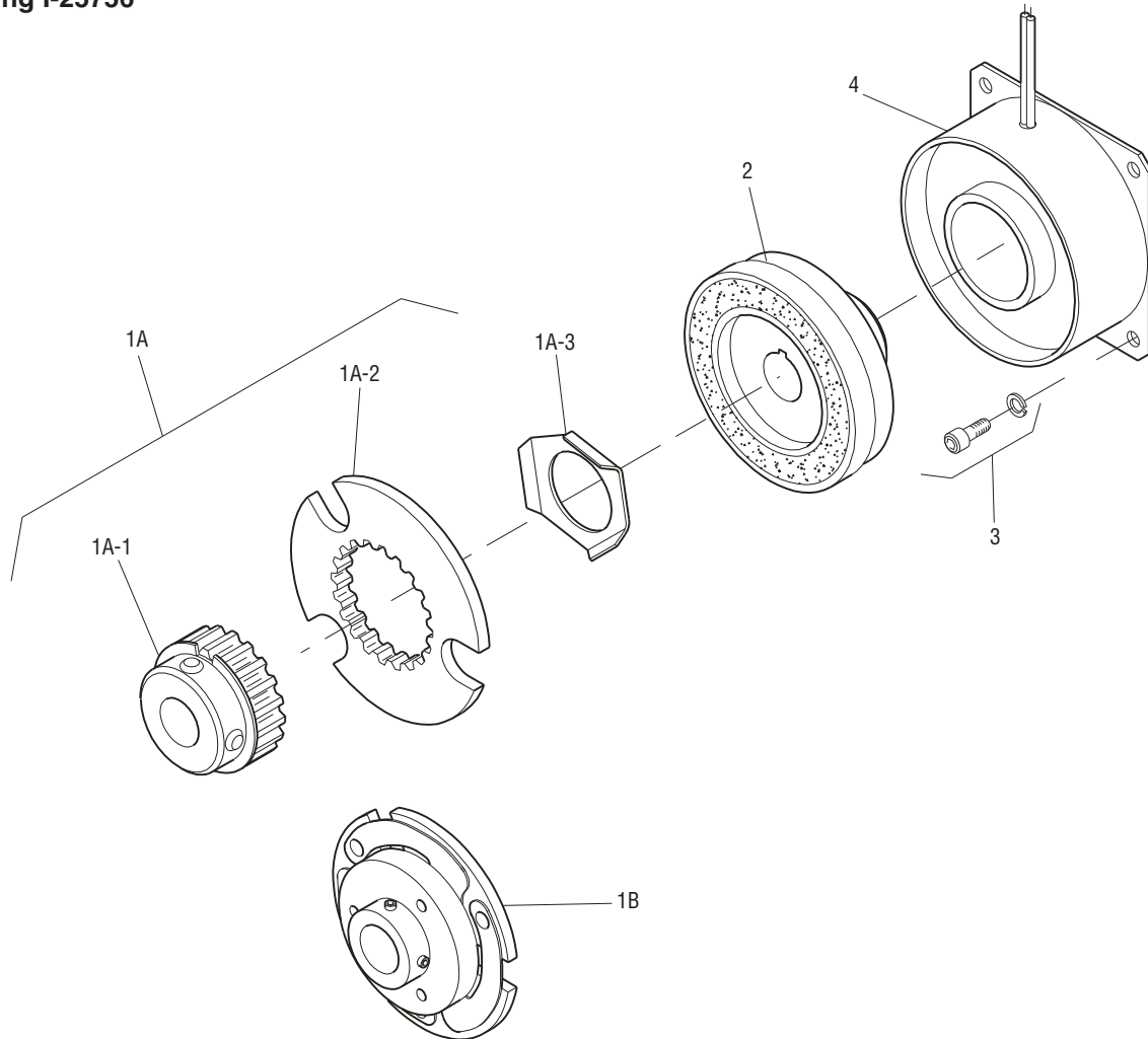
Drawing I-25756
