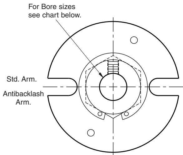
ARMATURE VIEW
