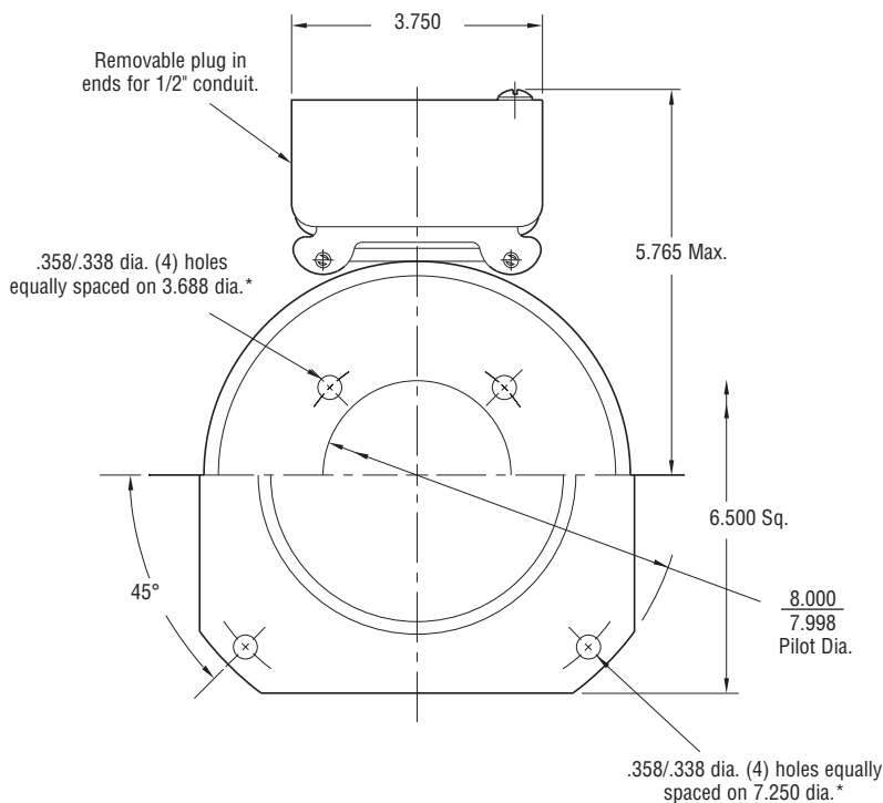
MAGNET VIEW (Inside & Outside Mounted)
