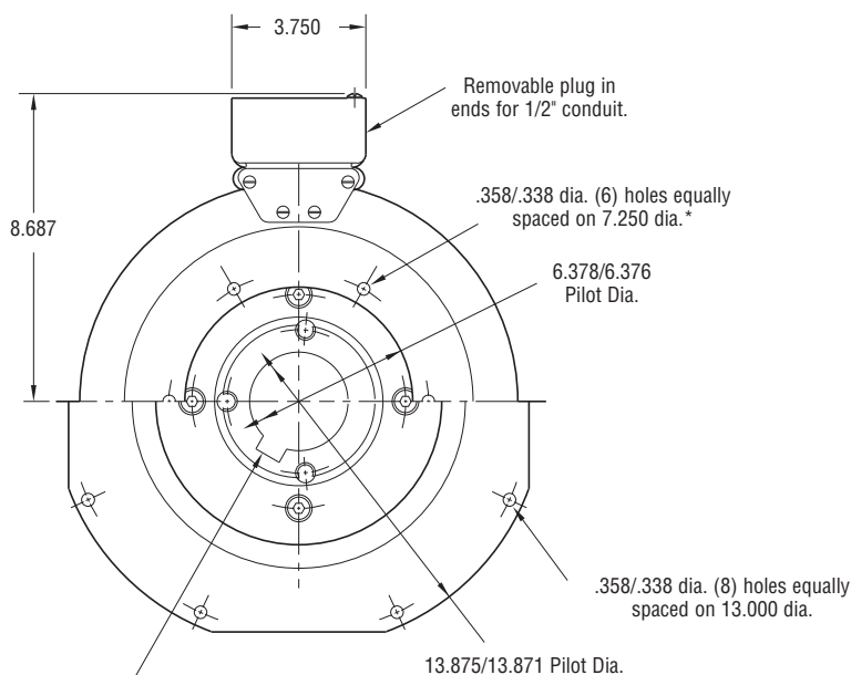
ARMATURE VIEW
