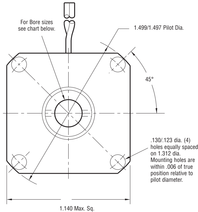
FIELD VIEW
