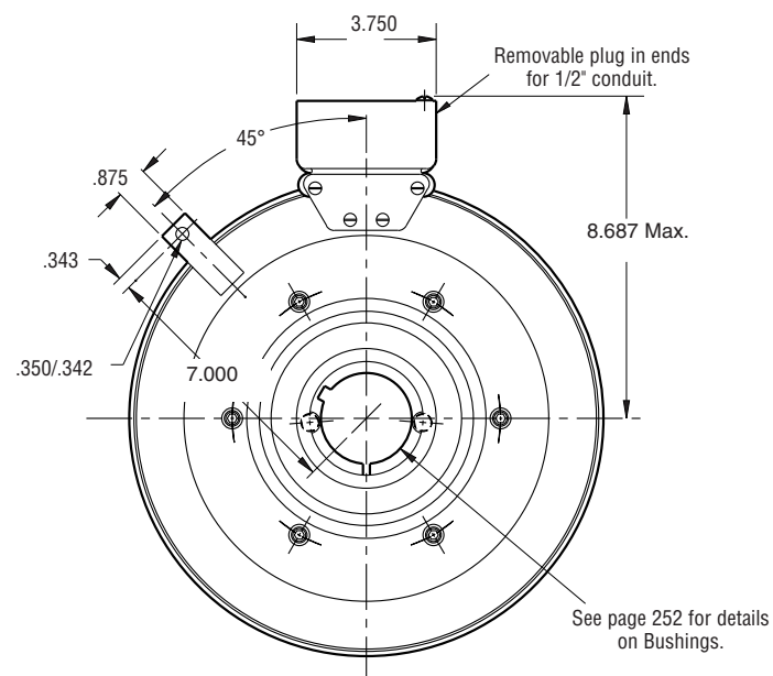
FIELD VIEW
