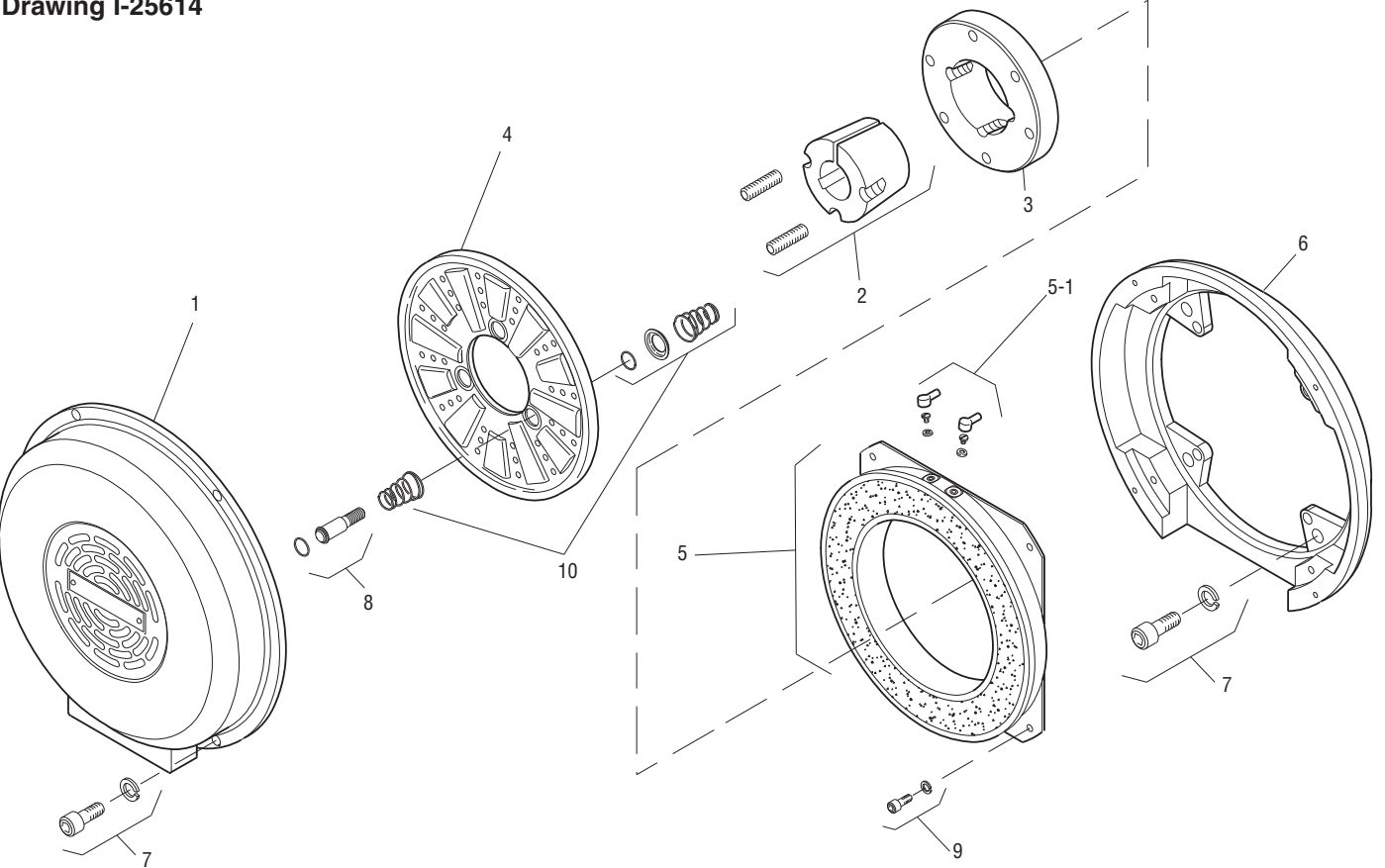
Drawing I-25614
